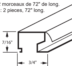
Moulure "Tri-Lite" Tri-Lite Window Snap Channel
