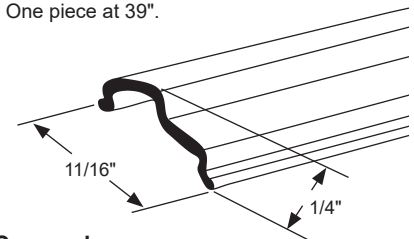
Couvercle Screw Cover Cap
